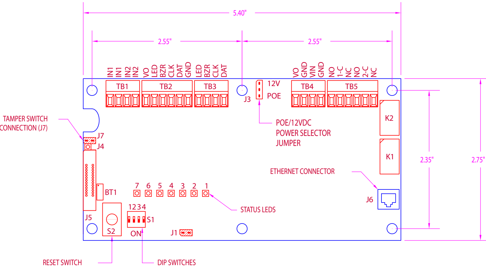
○ LNL-2210 INTELLIGENT SINGLE DOOR CONTROLLER SCALE: 1=1
